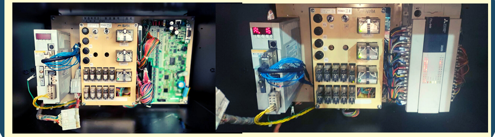
Upgrade PLC Main Board To PLC Fx-series
