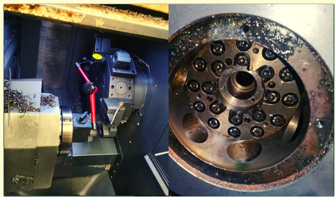
leveling & centering turret
