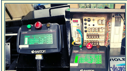
Modify Main Board To PLC
